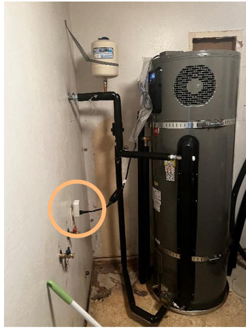
FIGURE 42. IMAGE SHOWING POWER METER PLUGGED INTO 120-VOLT OUTLET
