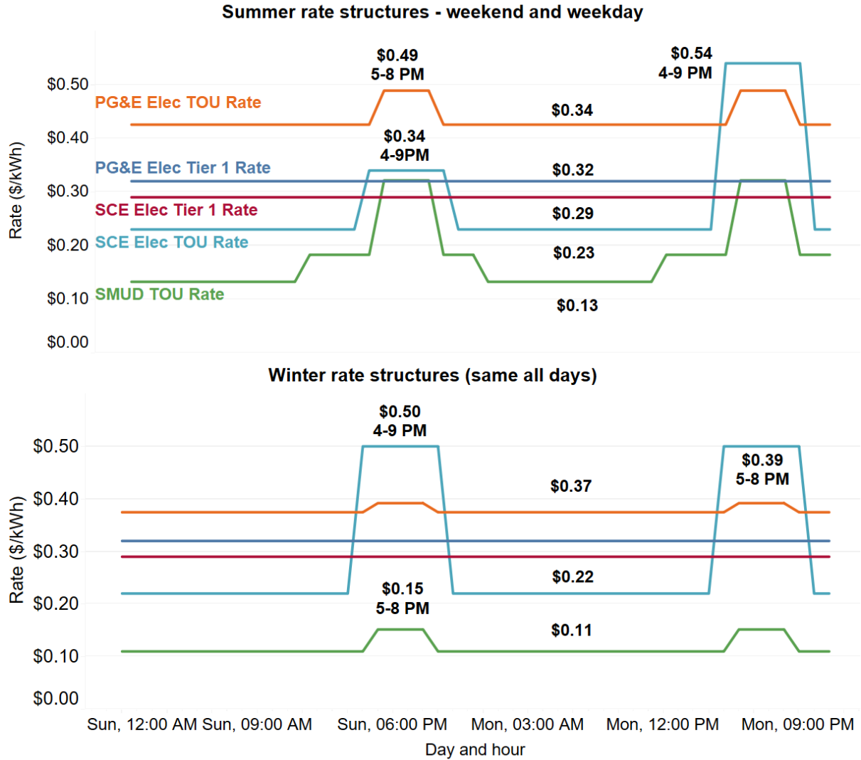
FIGURE 23. SUMMER AND WINTER ELECTRICITY RATE STRUCTURES FOR PG&E, SCE, AND SMUD
